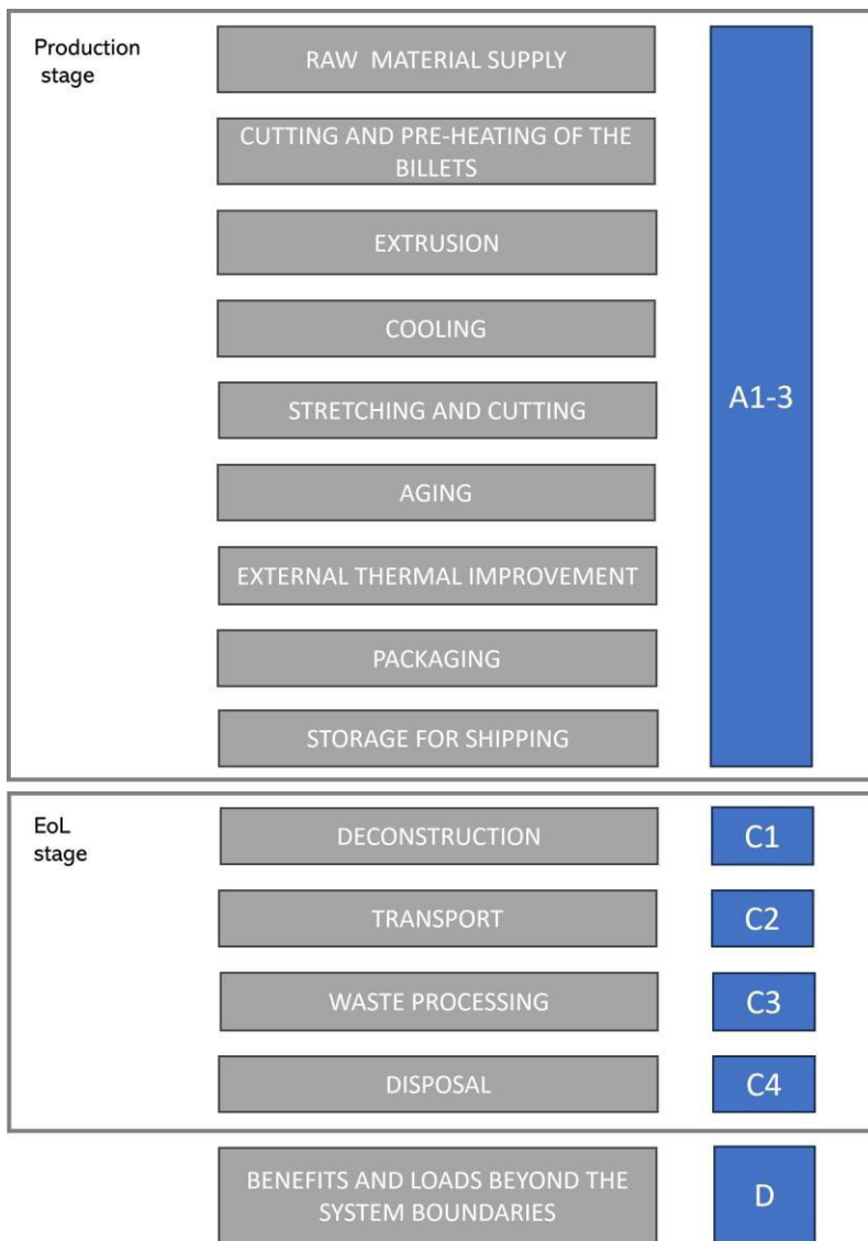
Figure 1. Scheme of the profiles manufacturing process occurring at Mississauga
